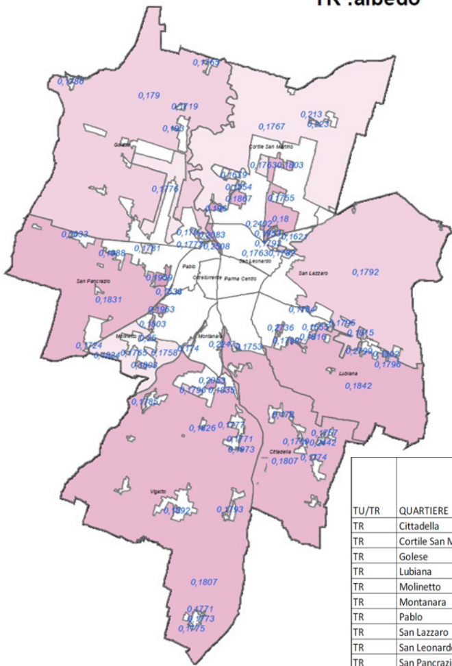
TR :albedo
