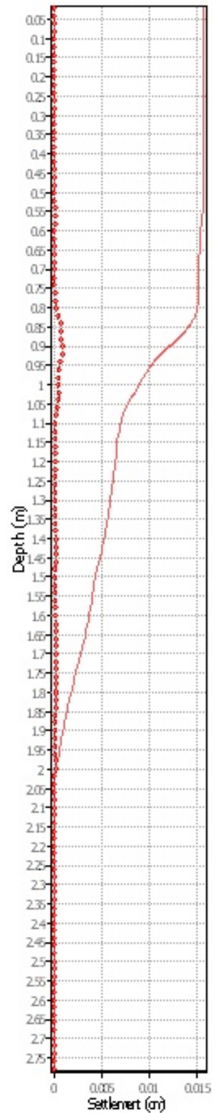
Vertical settlements
